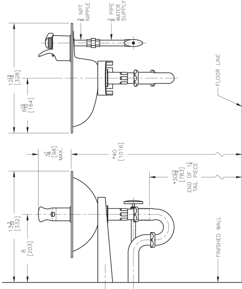
DIMENSIONAL DRAWING
